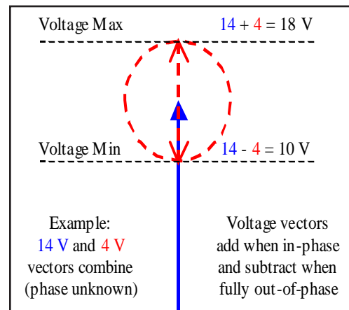
Fig. 3 Voltage Vectors
